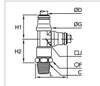
racor orientable
