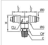
racor orientable
