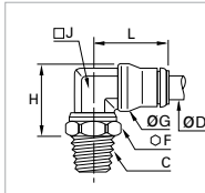
racor orientable
