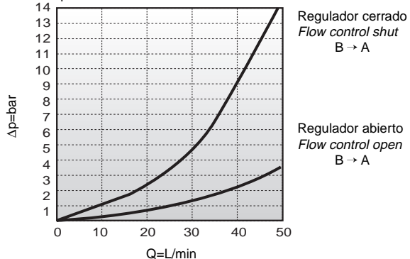
\Delta p - Q
