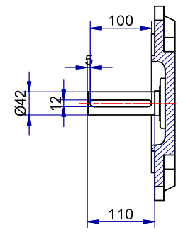
Shaft detail
