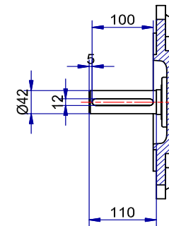
Shaft detail
