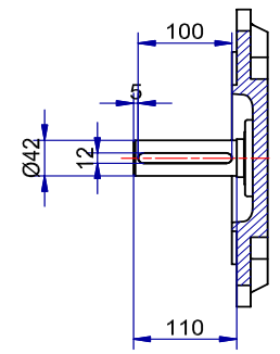
Shaft detail
