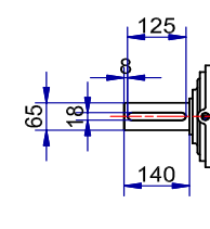
Shaft detail
