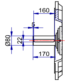
Shaft detail
