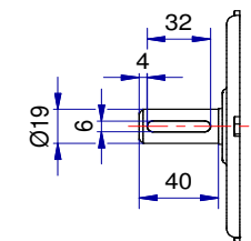
Shaft detail
