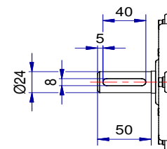
Shaft detail
